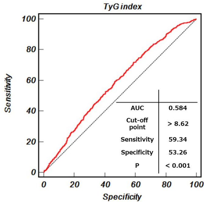
Fig. S1. The receiver operating characteristic curve pertaining to the triglyceride-glucose (TyG) index for moderate-to-severe chronic kidney disease. Dotted line, reference; solid red line, area under the curve (AUC), indicating the accuracy of the TyG index for the identification of moderate-to-severe chronic kidney disease; cutoff value, the value of TyG index that predicts moderate-to-severe chronic kidney disease; sensitivity, the probability of individuals who have moderate-to-severe chronic kidney disease to be predicted to have moderate-to-severe chronic kidney disease; specificity, the probability of individuals who do not have moderate-to-severe chronic kidney disease to be predicted not to have moderate-to-severe chronic kidney disease.
