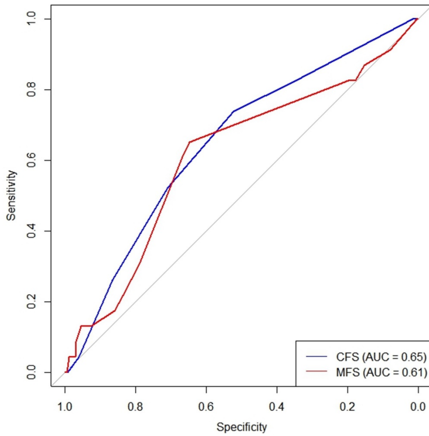
Fig. S3. Receiver operating characteristic curve for the fall risk assessment tool among participants aged 60 or more. CFS, Clinical Frailty Scale; MFS, Morse Fall Scale; AUC, area under the curve.
